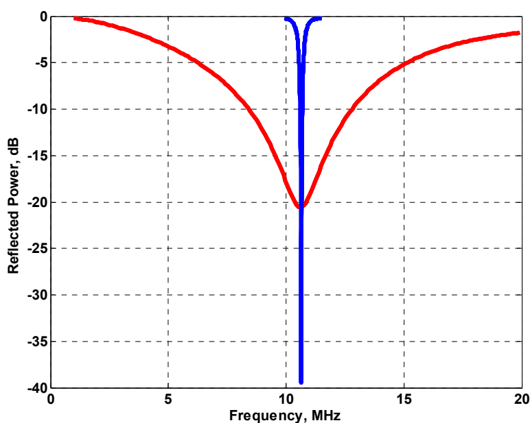
Figure 3. The resonance curves for the fabric coil probe (red line) and the NMR MOUSE™ probe (blue line).
